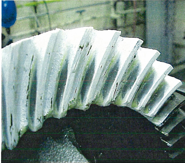
Before Test Contact Pattern
