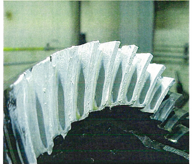
After Test Contact Pattern
