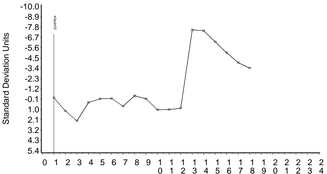
CUSUM Severity Analysis
