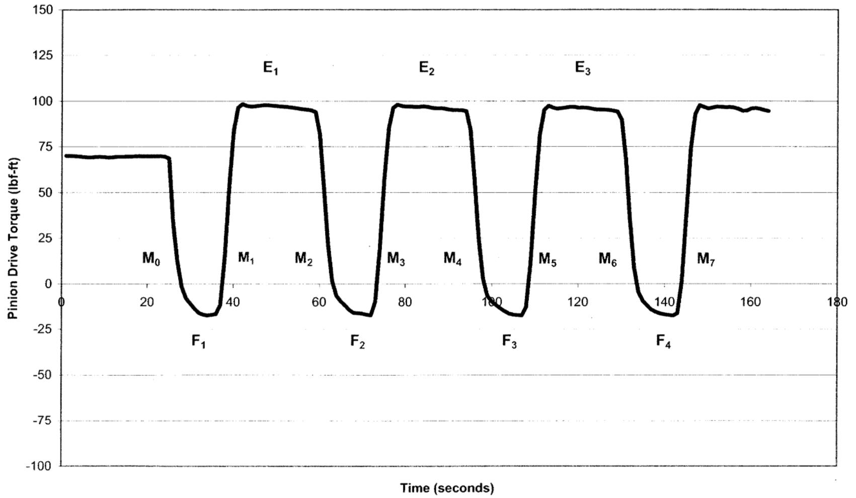
FIG. A2.18 Conditioning 4 – Pinion Torque (Exploded View)
