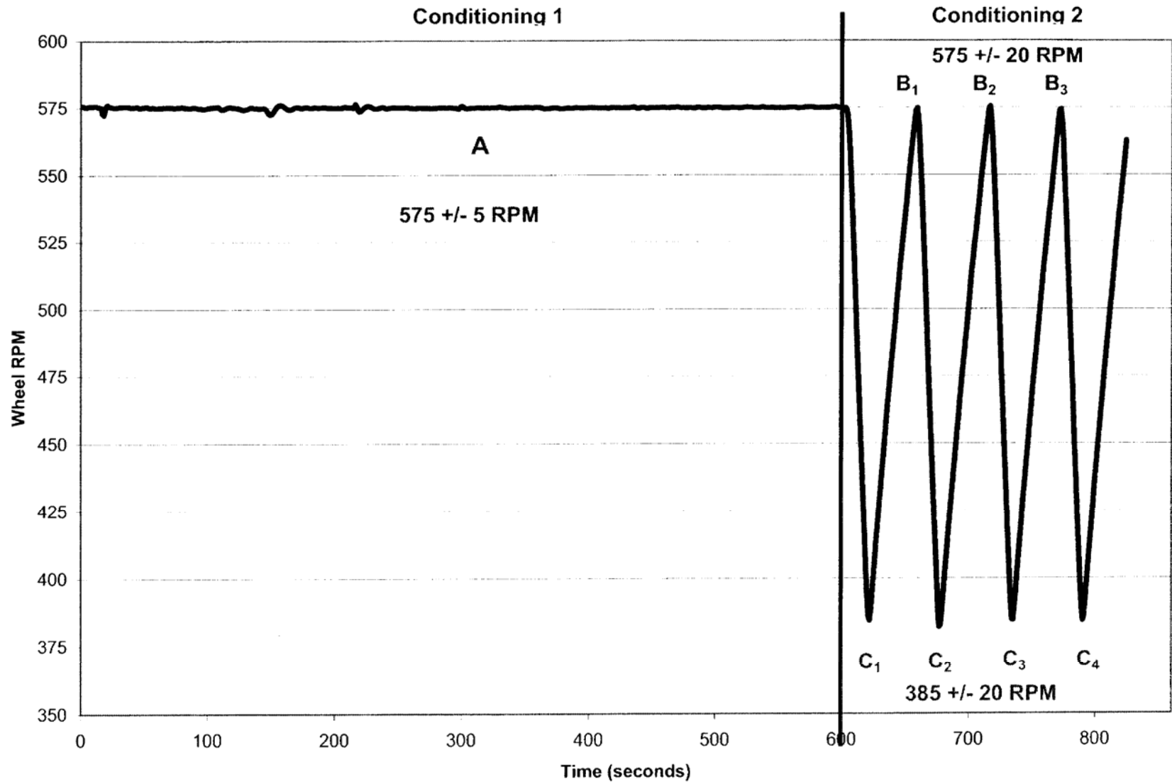
FIG. A2.11 Conditioning 1 & 2 - Wheel Speed
