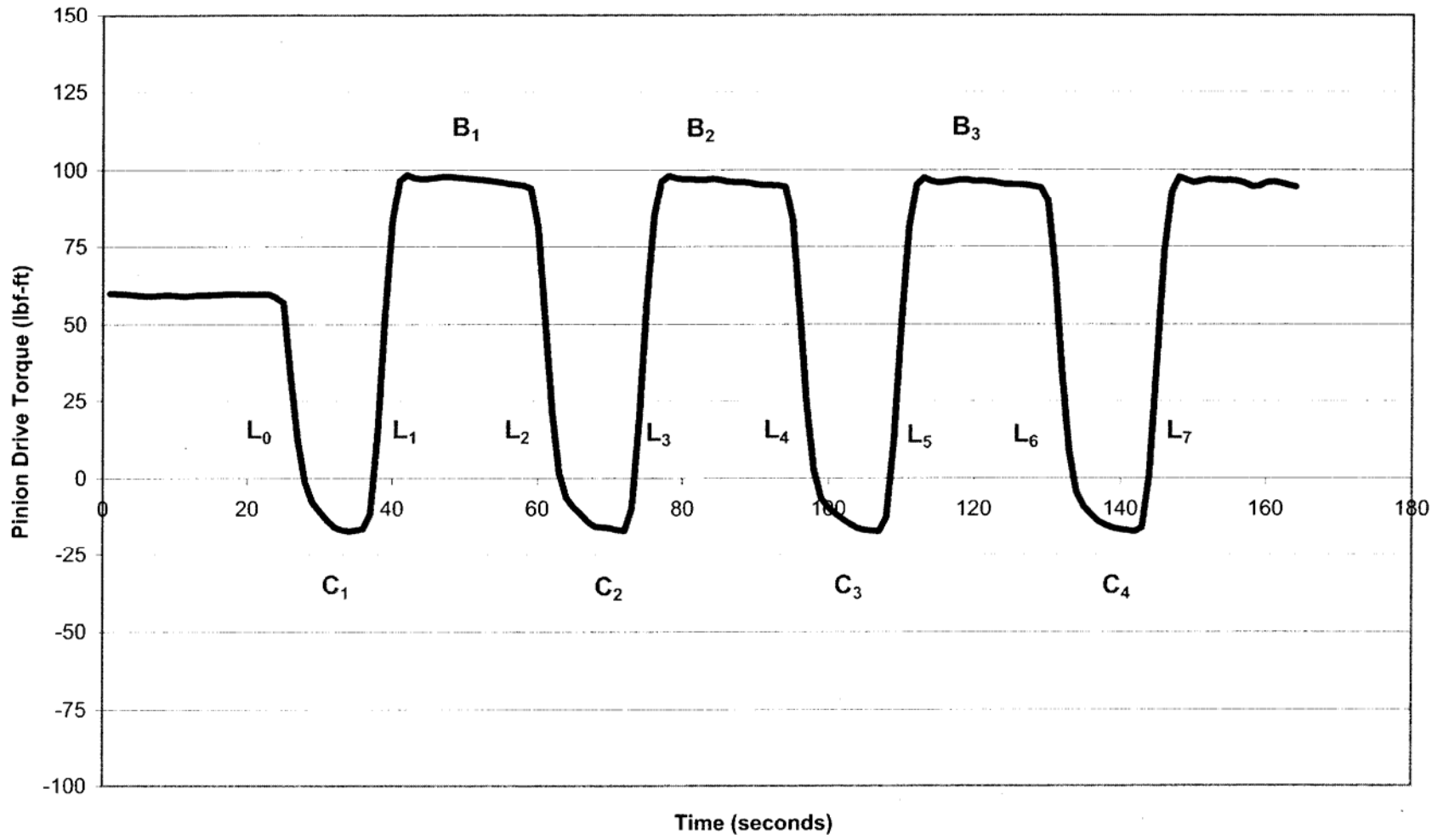
FIG. A2.17 Conditioning 2 – Pinion Torque (Exploded View)
