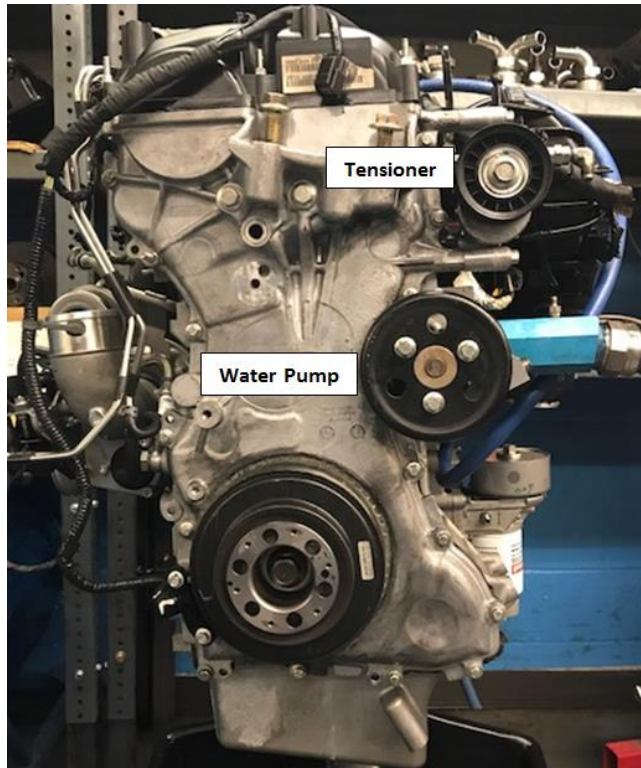
FIG. 2 Water Pump Drive Arrangement
