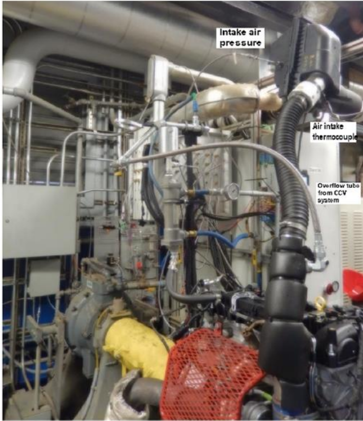
FIG. A9.12 Typical air intake system
