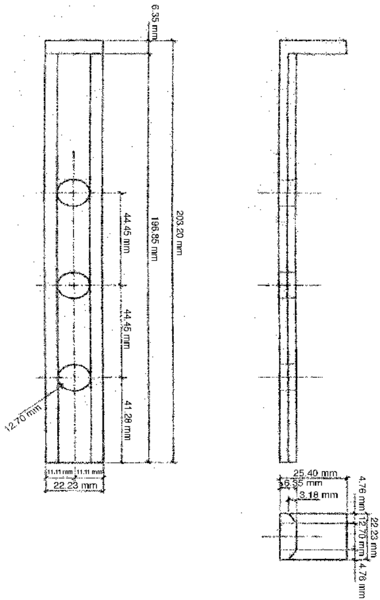
Fig. A7.2: Cylinder Bore Ladder
