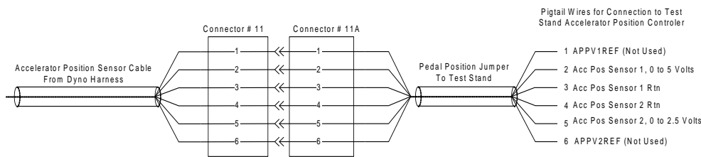
Figure 13: Accelerator Position Wiring Schematic
