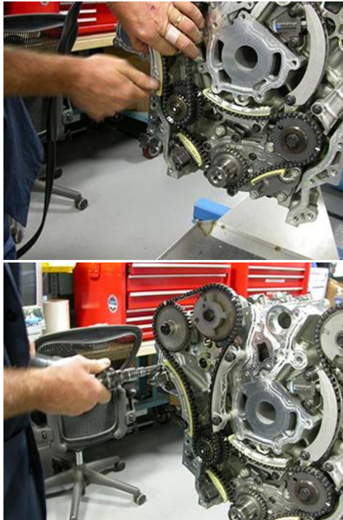
FIG. A17.18 View Showing Chain Guide and Tensioner Installation
