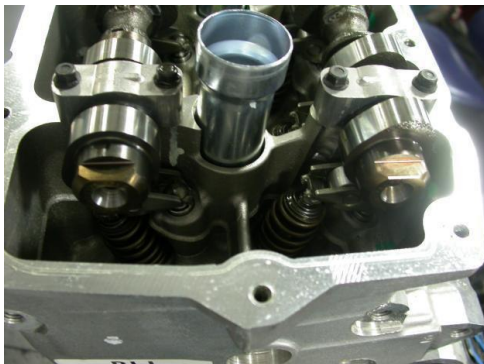
Fig A17.1 Cam Positioning
