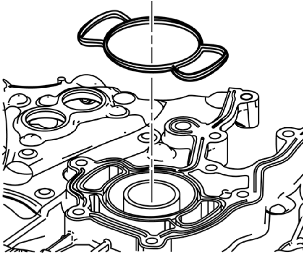
FIG. A17.23 Location of Front Cover Seal
