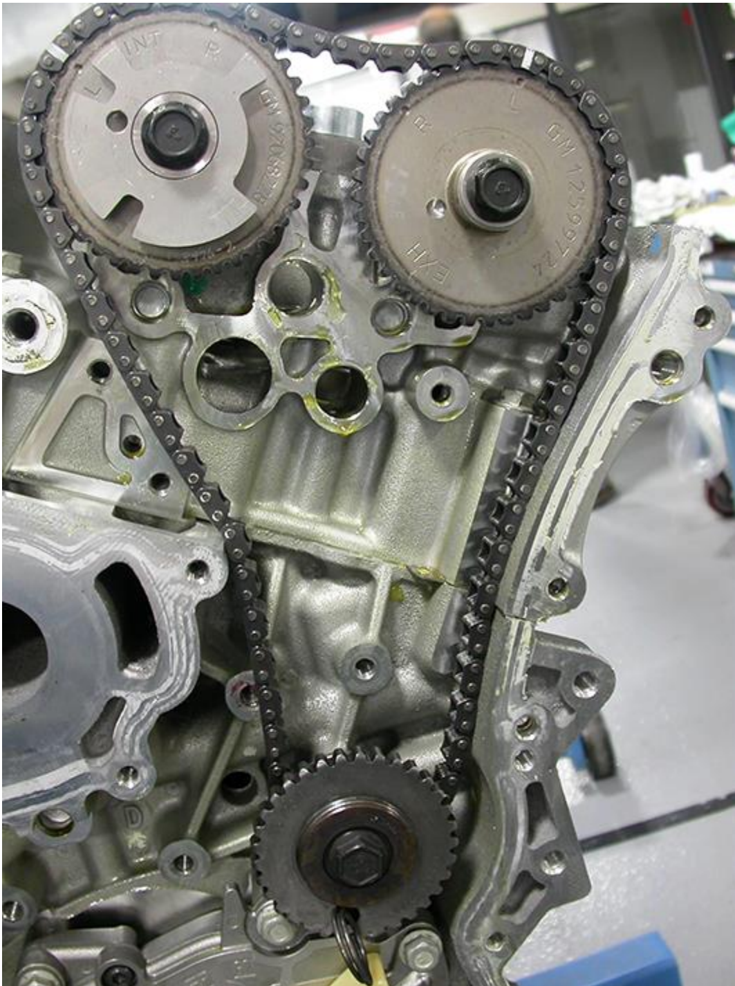
FIG. A17.10 Alignment of Timing Marks, Left Side, with Grenade Pin Installed
