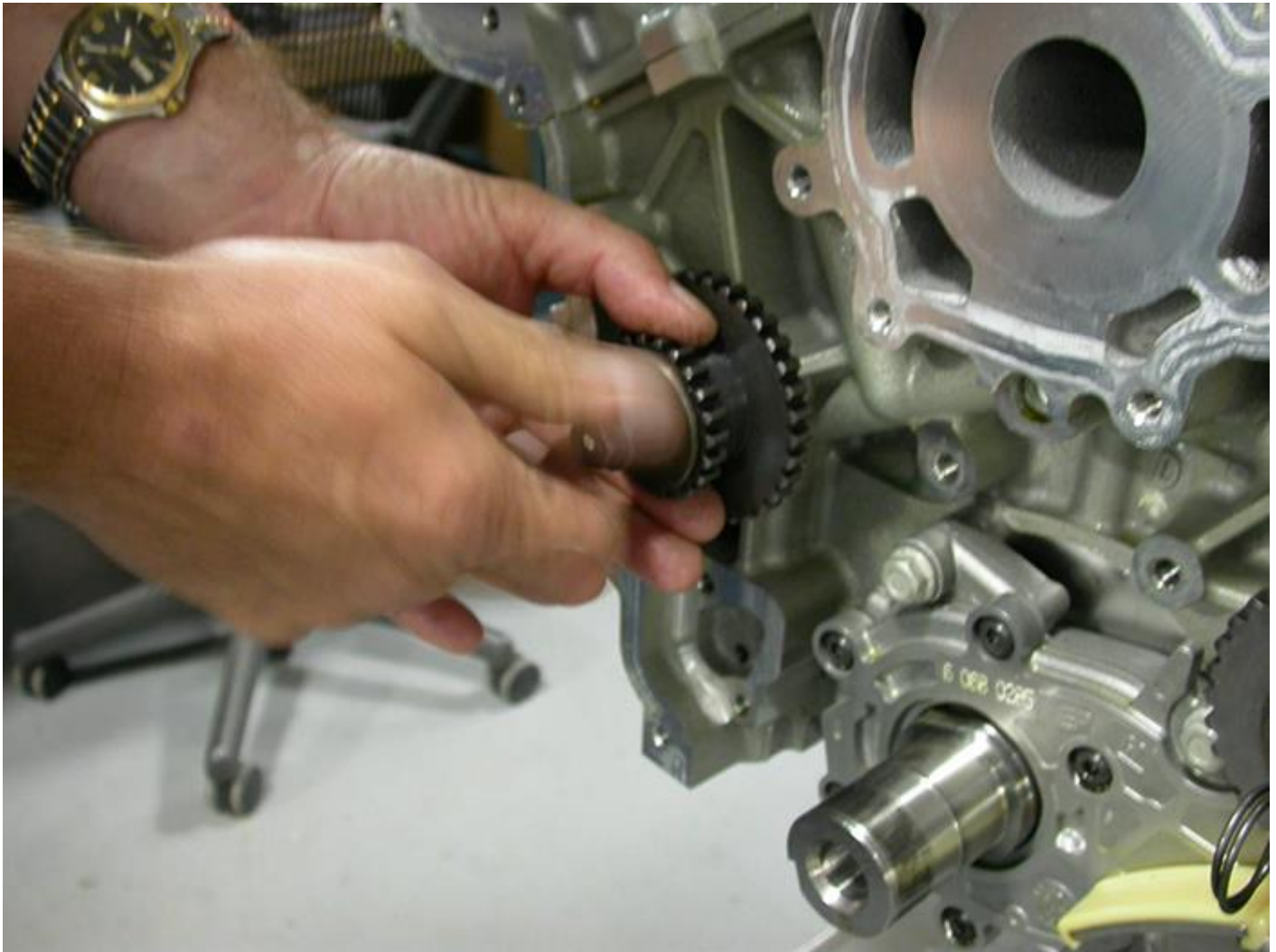
FIG. A17.12 Installation of Right Side Idler Gear
