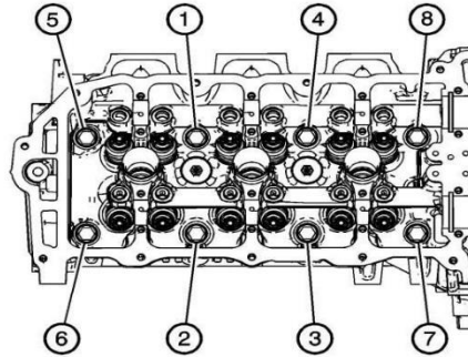
Fig A17.6 Torquing Sequence for Left Cylinder Head
