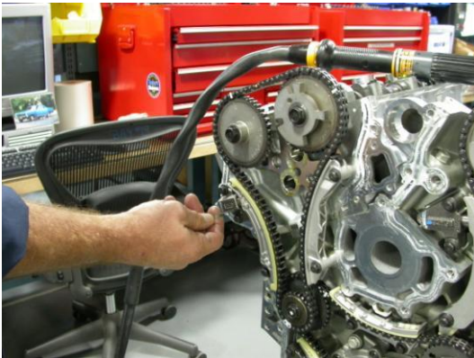
Remove grenade pin from right side chain tensioner.
