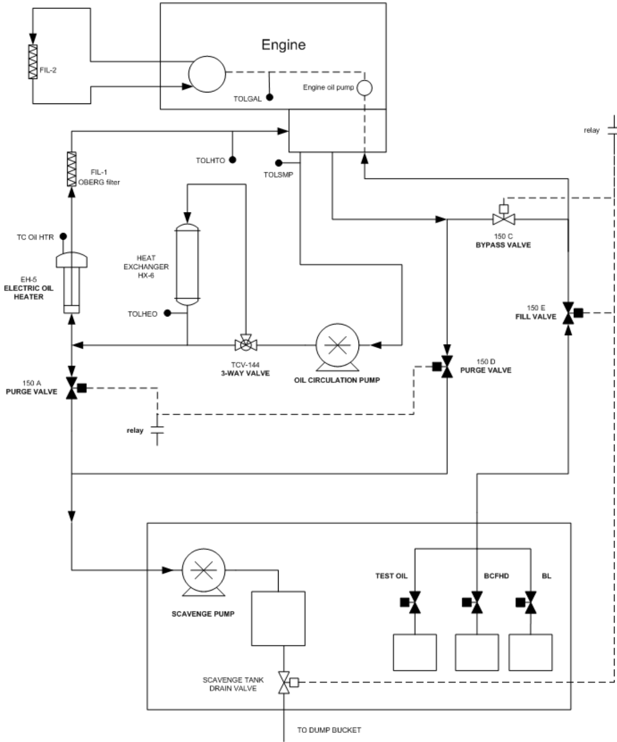
FIG. A2.6 External Oil System
