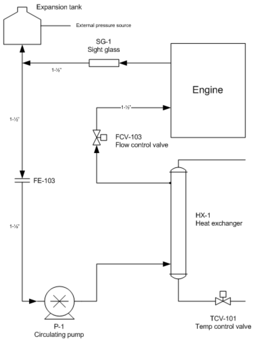
FIG. A2.2 Alternate Cooling System
