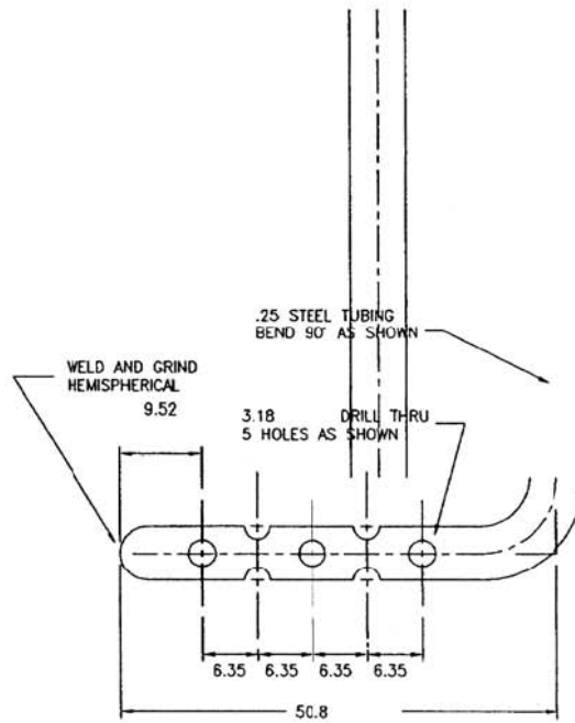
PROBE DETAIL
