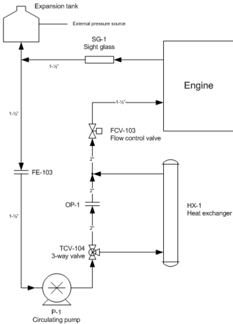
Fig A2.1 Typical Engine Cooling System
