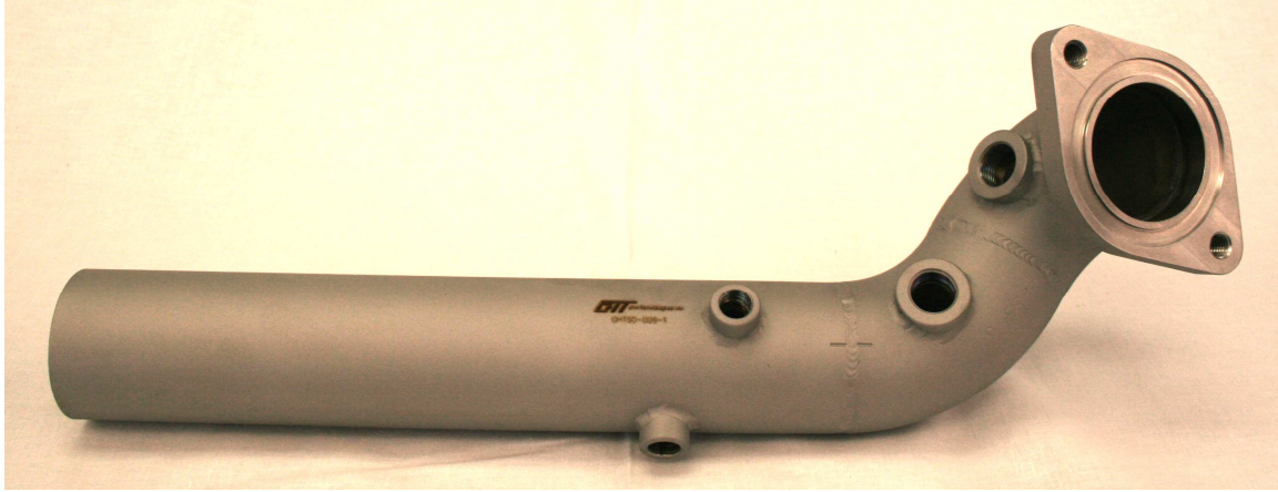
FIG. A2. 14 TAKE DOWN TUBE, R.H. ASSY.
