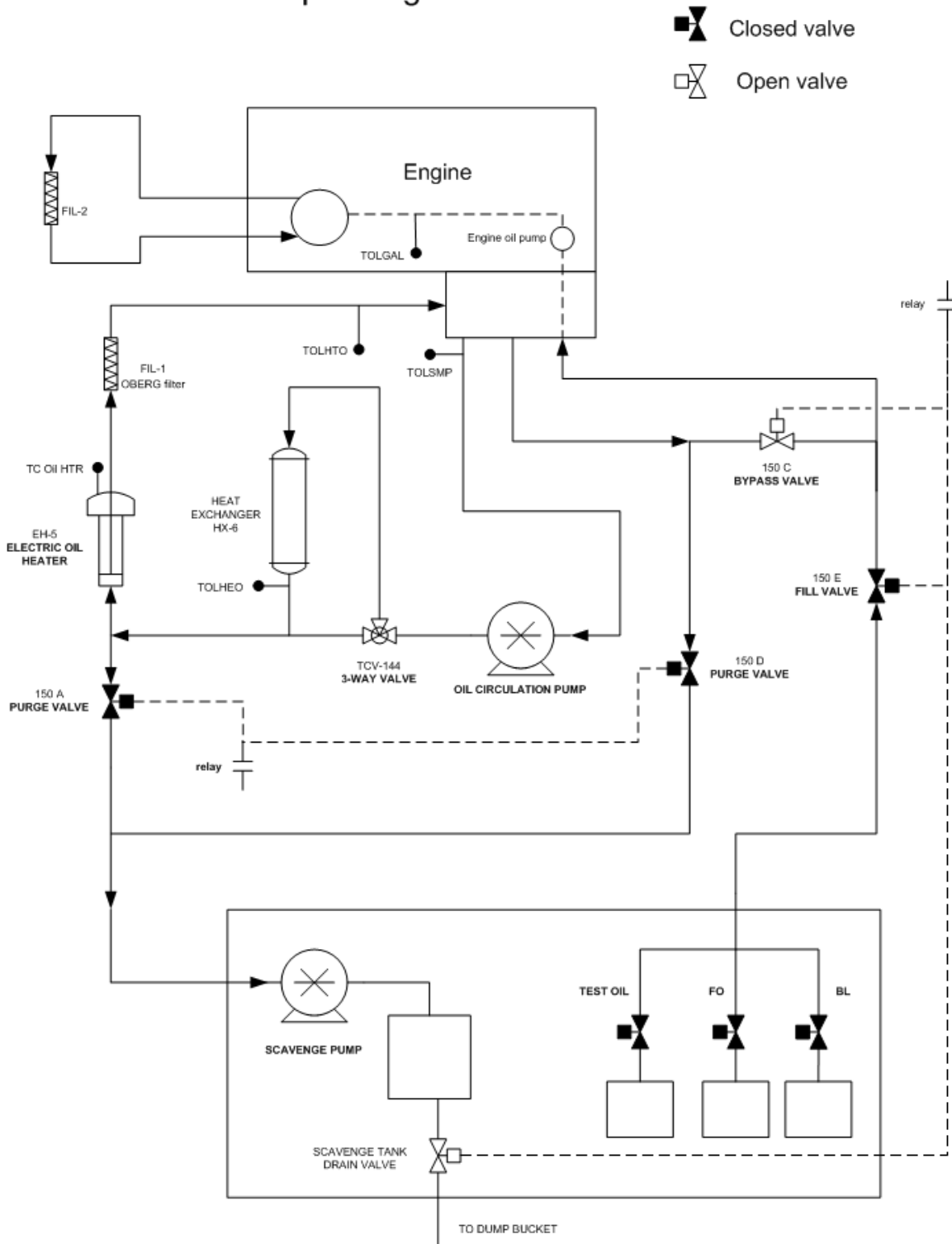
FIG. A2.6 External Oil System
