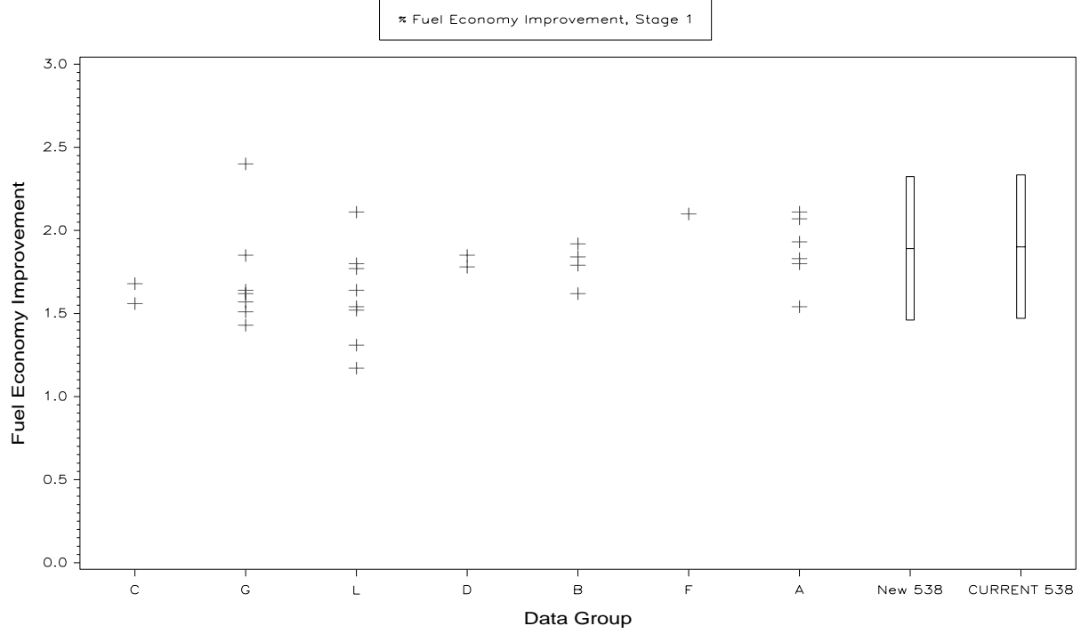
Sequence VIB (Reference Oil 538) Test Target Data Set and Shewart Severity Limits
