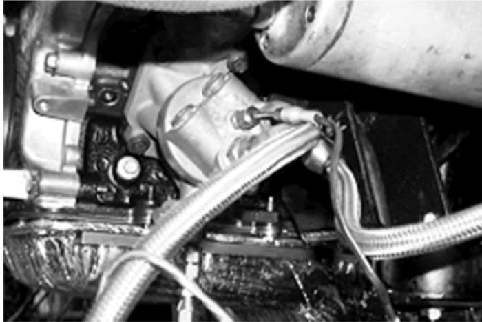
FIG. A7.25 Oil Cooling System, Adapter Housing at the Engine with Typical Fittings for Temperature Sensors, Pressure Tap and Oil Filter
