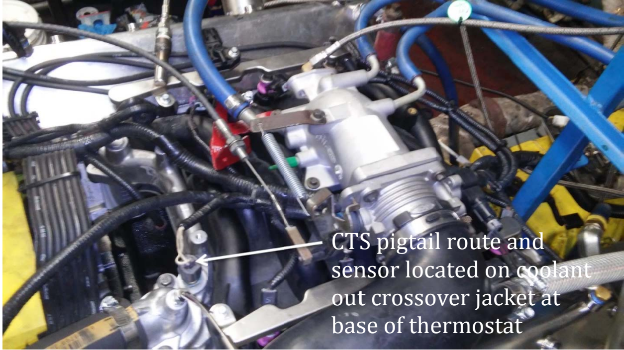
FIG A7.36 New style coolant temp sensor wire routing.
