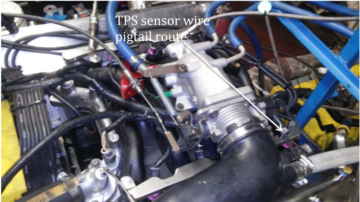
FIG A7.34 Throttle Position Sensor wire routing on test engine
