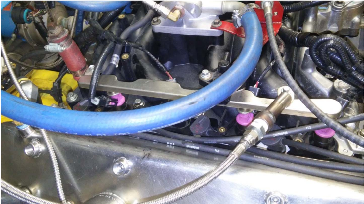
FIG A7.29 Bank one injector wire route without plastic shield
