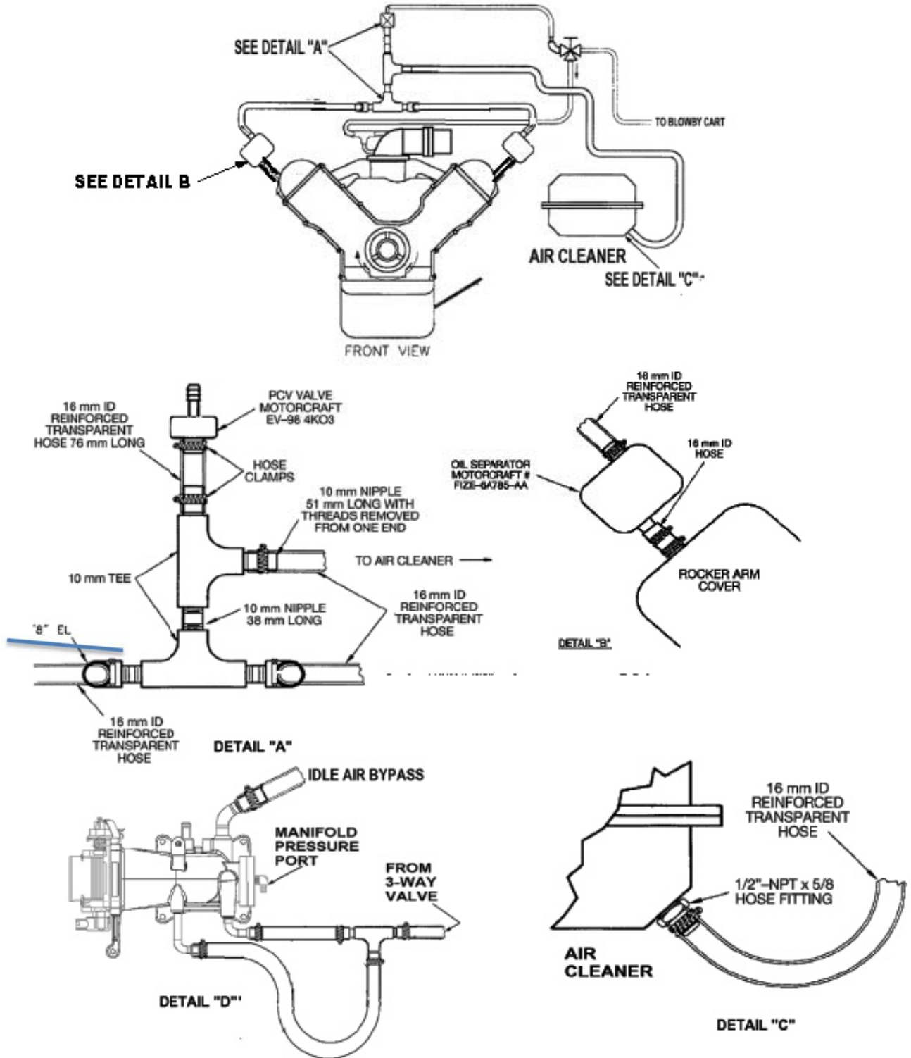
FIG. A7.17 Closed Crankcase Ventilation System, Typical Fittings and Parts Configuration
