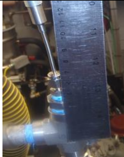
Figure A7.14 Blow-by Gas Out
