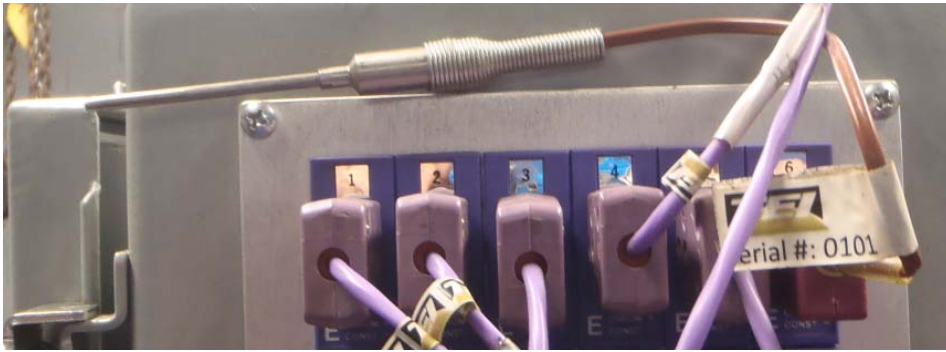
Figure A7. 6 Test Cell
