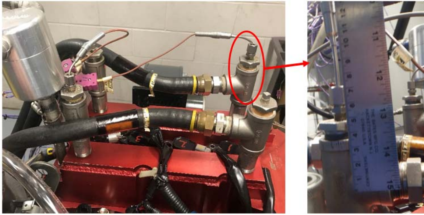
Fig. A7. 10 Valve Cover Coolant In
