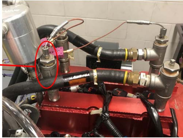
Figure A7.11 Valve Cover Coolant Out
