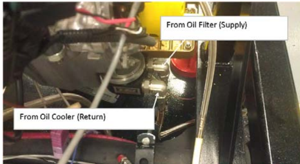
Fig. 2 Remote Oil Filter Housing Adapter
