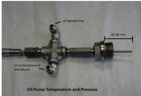
FIG. A2.8 Oil Pump Temperature and Pressure
