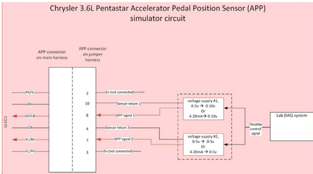
FIG. A11.1 Block Diagram for Chrysler 3.6 L Pentastar Accelerator Pedal Position Simulator Circuit
