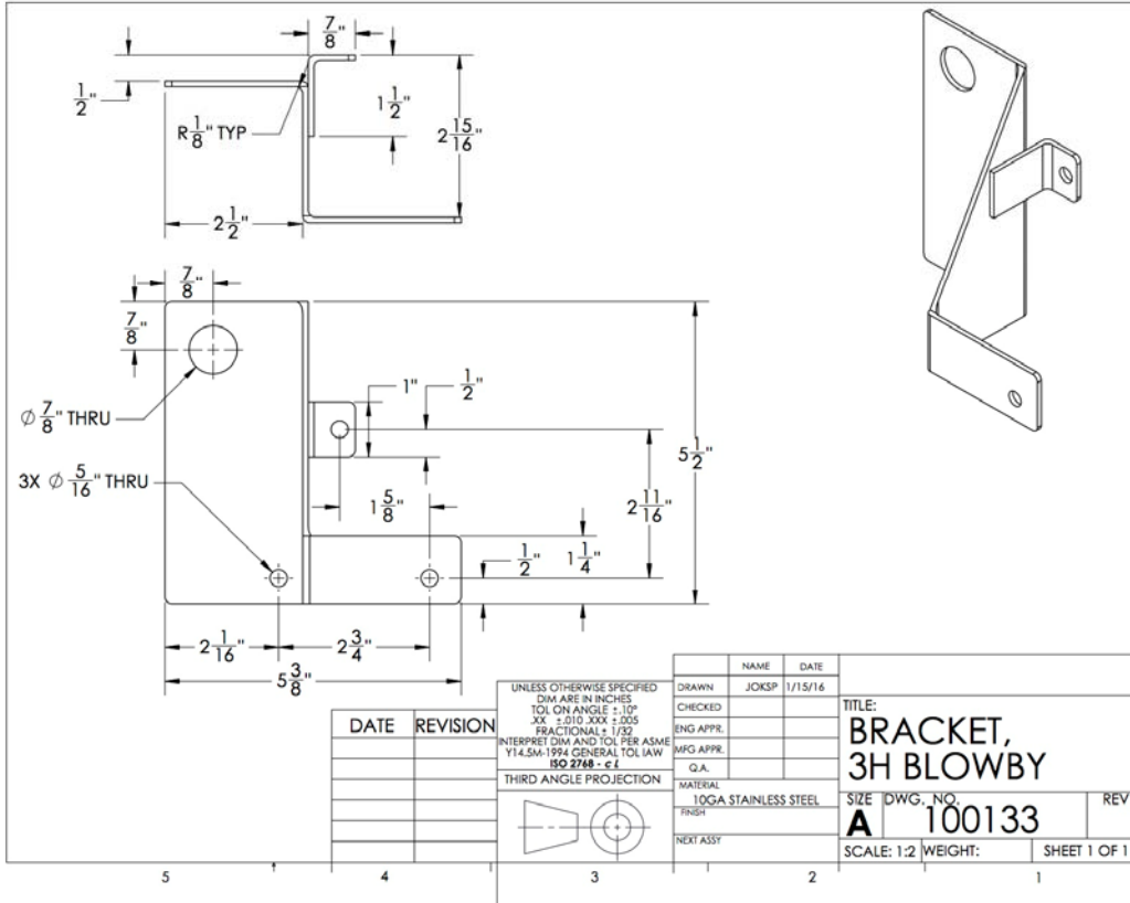
FIG. A3.2 Blowby Ventilation Support Bracket
