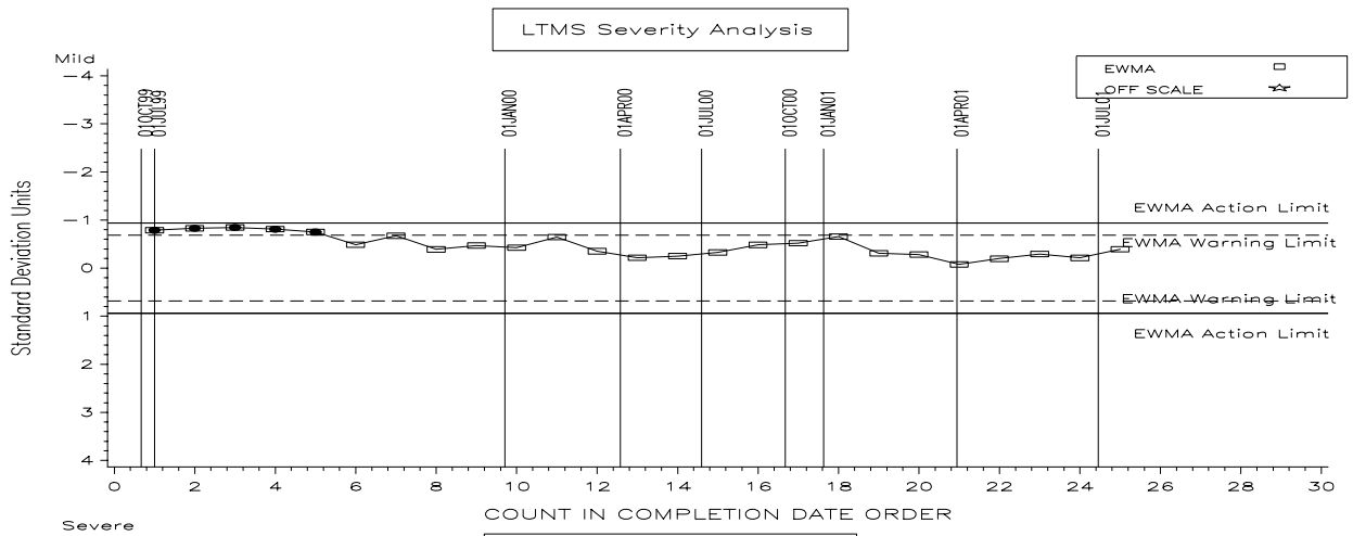
FIGURE 2 T-8/T-8E INDUSTRY OPERATIONALLY VALID DATA VISCOSITY INCREASE AT 3.8% SOOT (CST)
