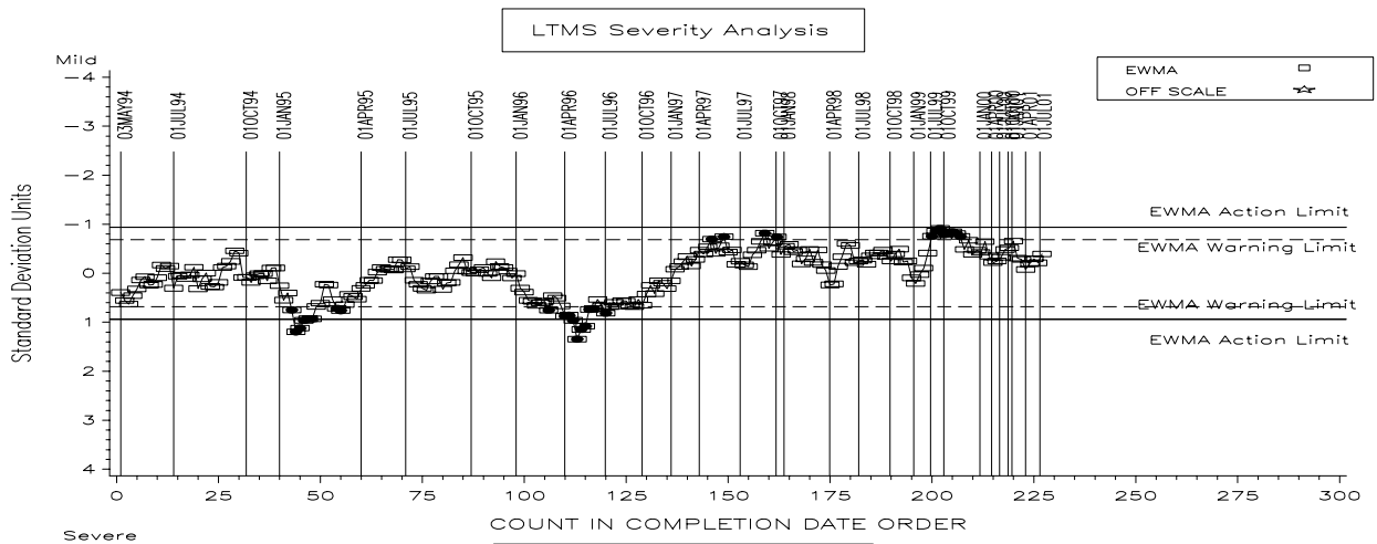
FIGURE 1 T-8/T-8E INDUSTRY OPERATIONALLY VALID DATA VISCOSITY INCREASE AT 3.8% SOOT (CST)
