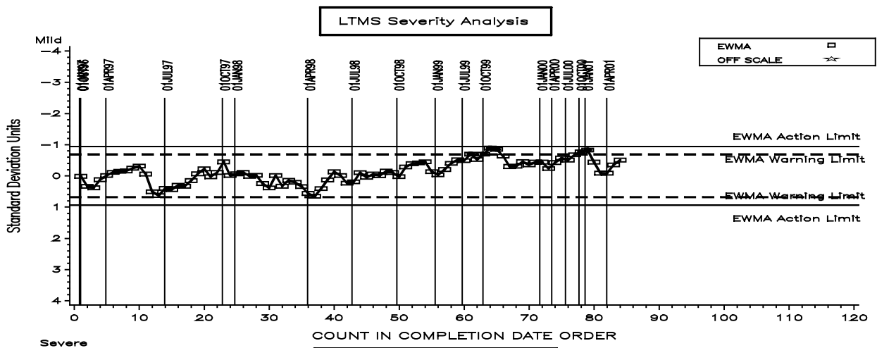
FIGURE 3 T-8/T-8E INDUSTRY OPERATIONALLY VALID DATA RELATIVE VISCOSITY AT 4.8% SOOT
