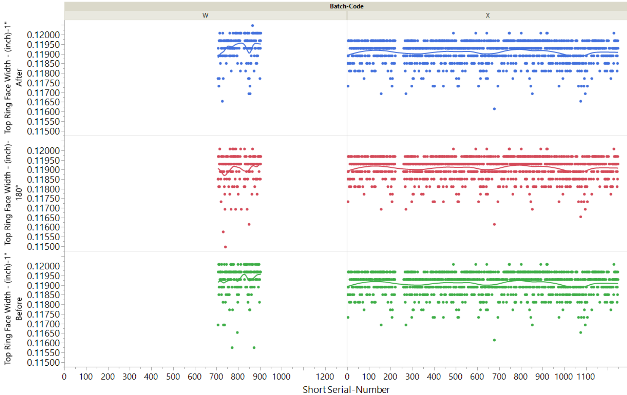
Top Ring Face Width - (inch)-1" Before & 2 more vs. Short Serial-Number
