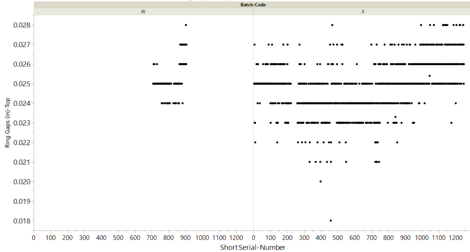
Ring Gaps (in)-Top vs. Short Serial-Number
