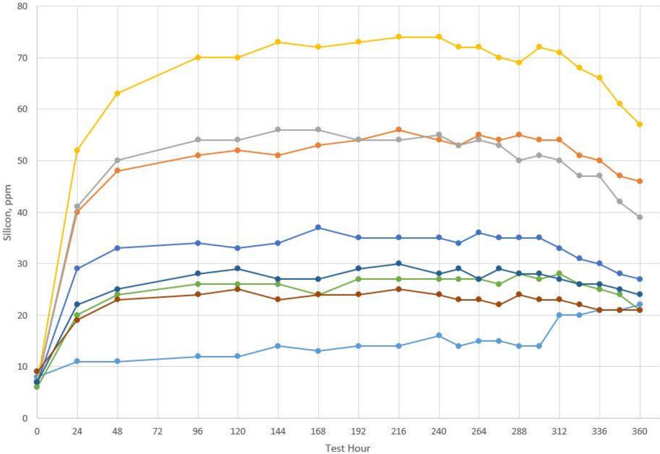
T13 Ref Oil 823 w/ Humidity Dew Point Control
