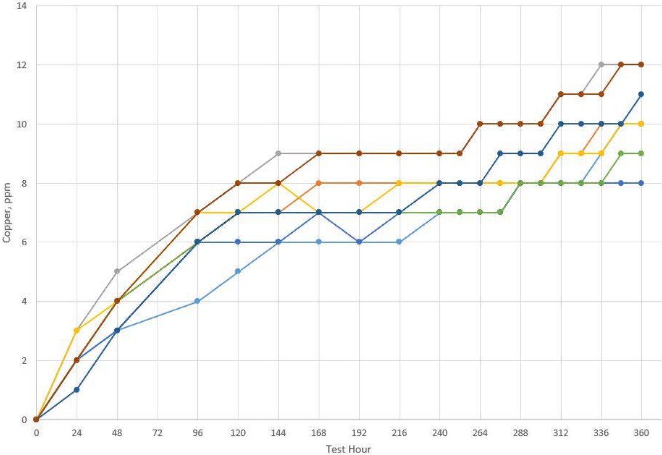
T13 Ref Oil 823 w/ Humidity Dew Point Control
