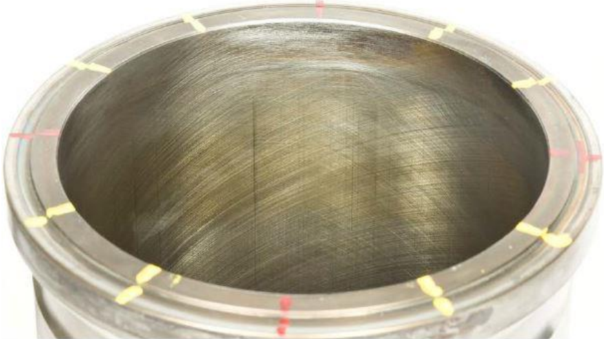
ANTI-THRUST
