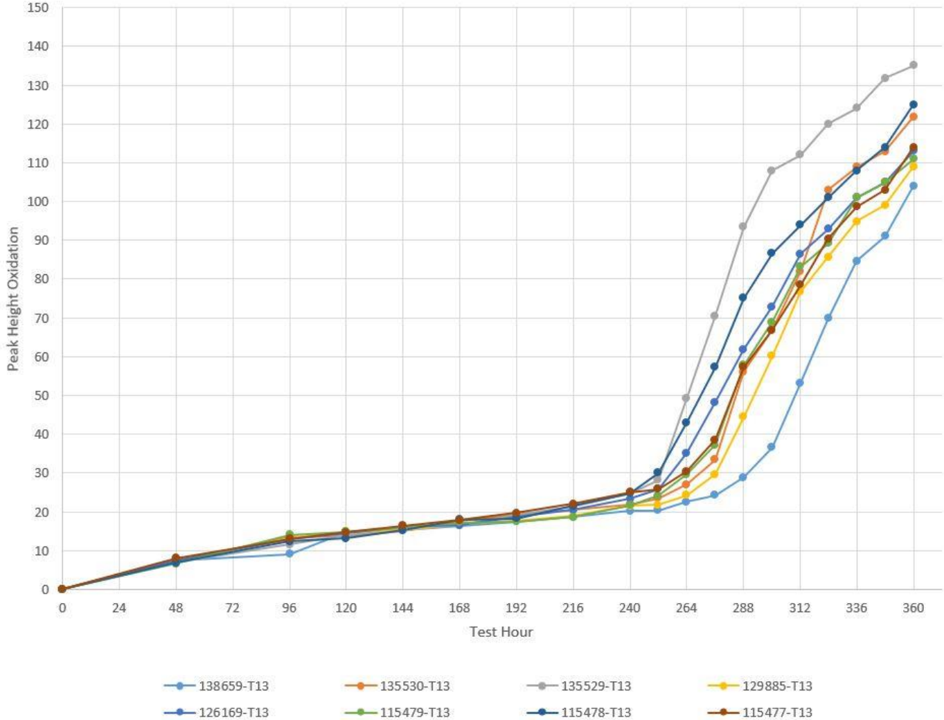
T13 Ref Oil 823 w/ Humidity Dew Point Control
