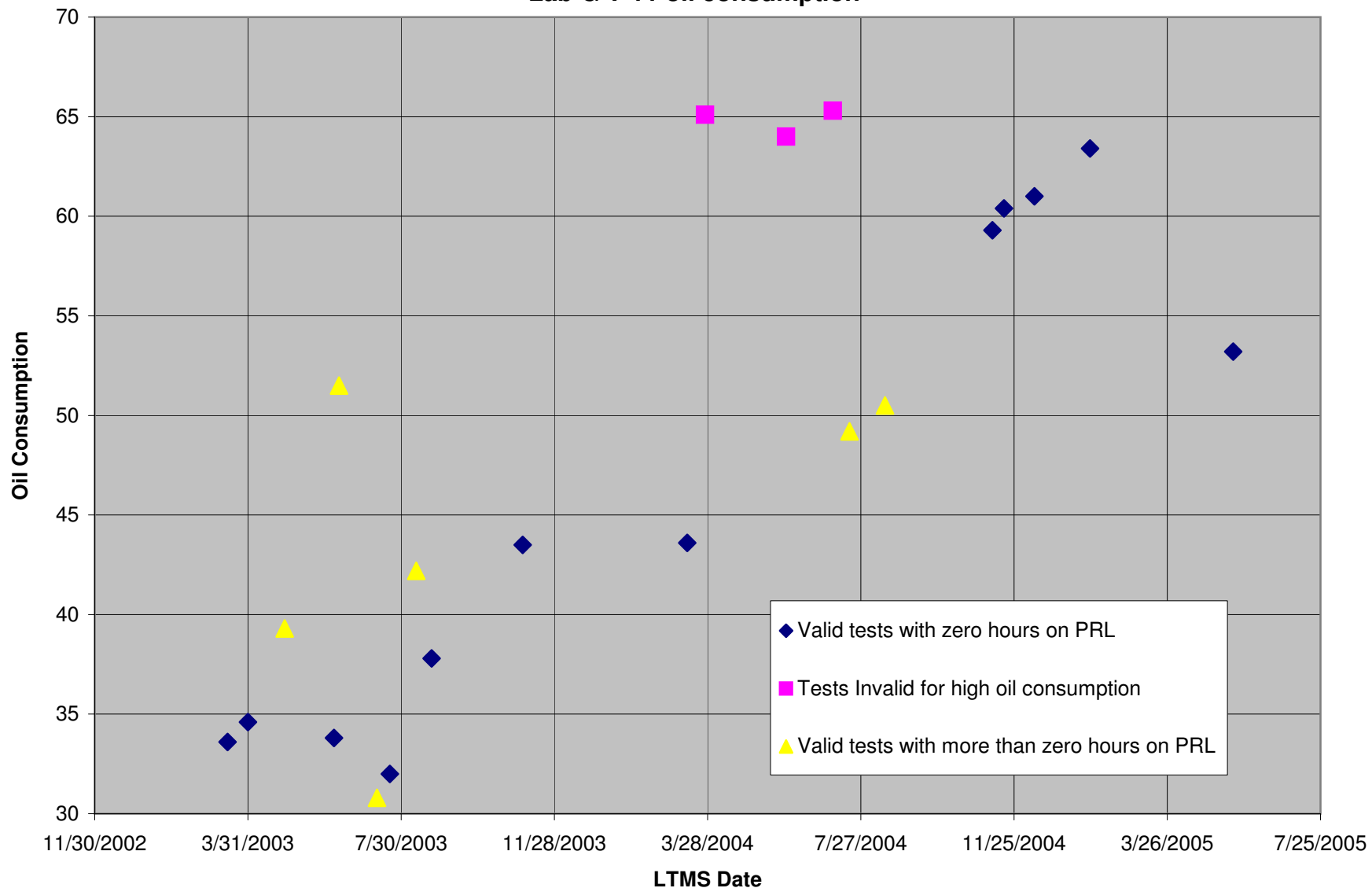
Lab G T-11 oil consumption
