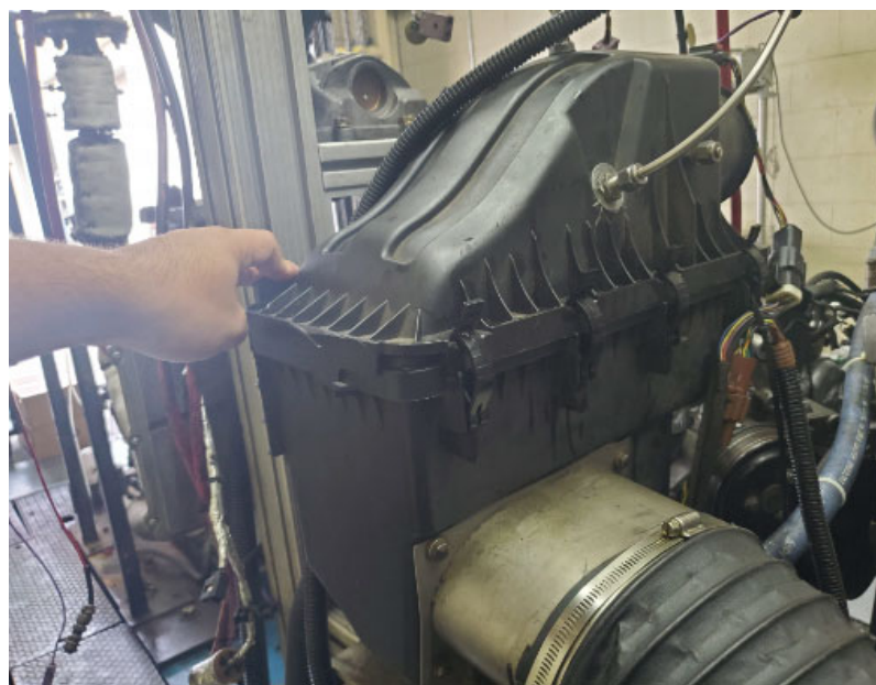
Figure A4.38 Modified Production Air Box
