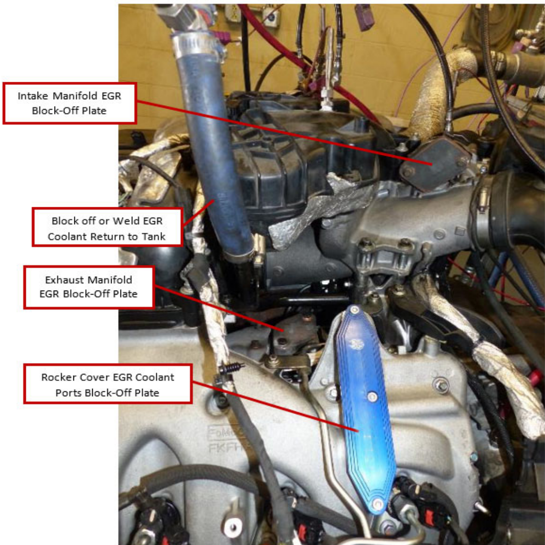
Figure A4.9 EGR System Modifications
