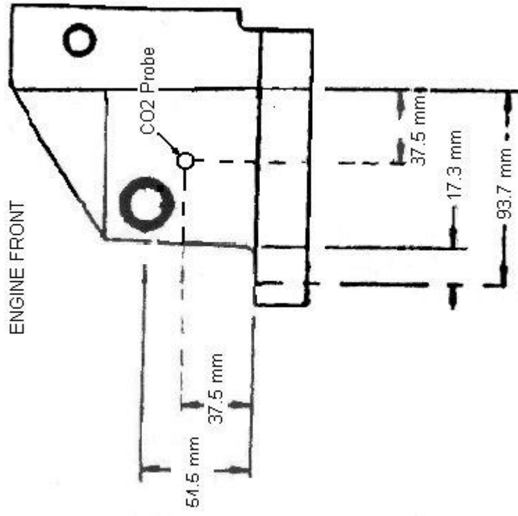
Figure A4.13 Intake Manifold CO2 Probe Location
