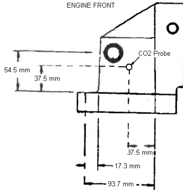
Figure A4.14 Intake Manifold CO2 Probe Location
