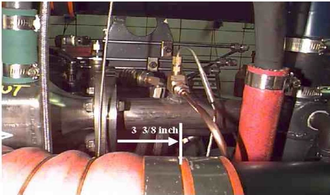
Update on tube from exh. To EGR Cooler pn y4006151 Rev 7/21/99
