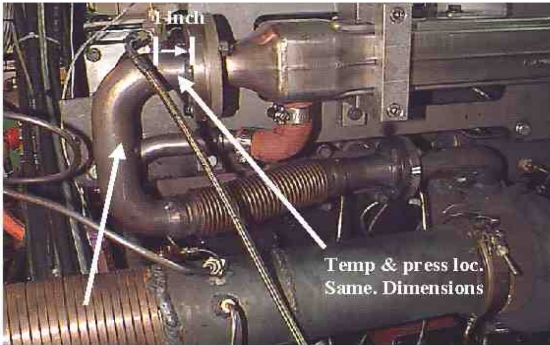
Update on tube from exh. To EGR Cooler pn y4006151 Rev 7/21/99
