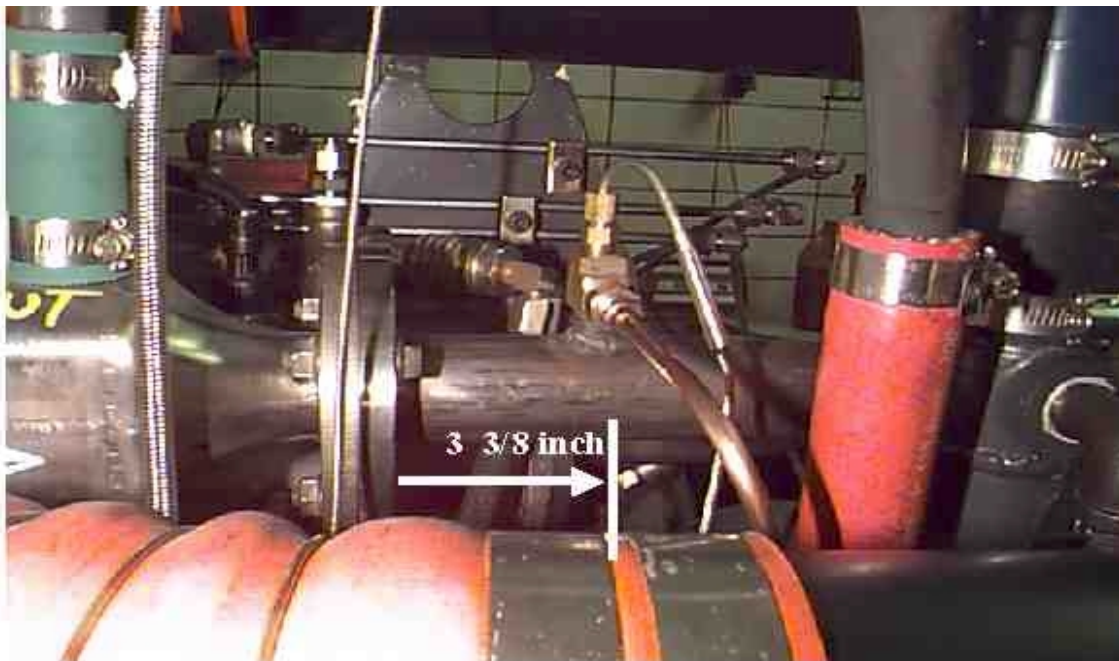
Update on tube from exh. To EGR Cooler pn y4006151 Rev 7/21/99
