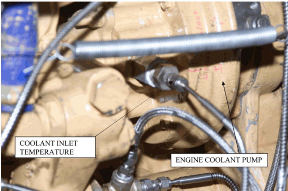
FIG. A5.14 Coolant to Engine
