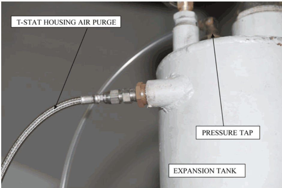
FIG. A5.18 Cooling-System Pressure Measurement
