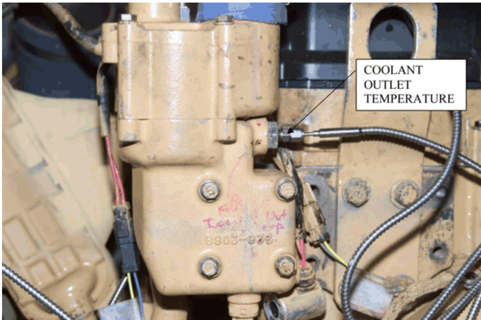
FIG. A5.13 Coolant-Outlet Temperature
