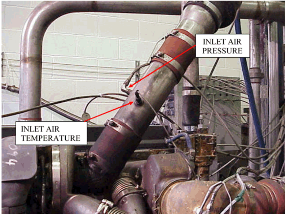
FIG. A5.7 Inlet Tube
