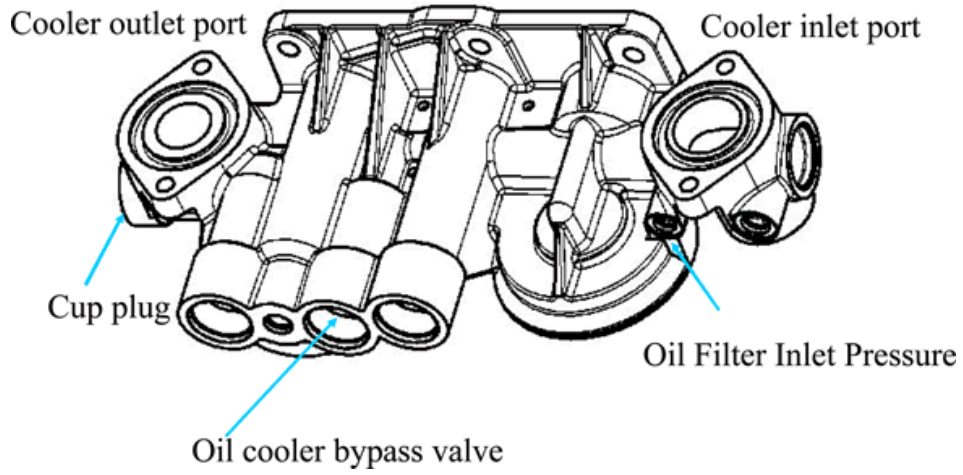
FIG. A4.2 Filter Base (P/N 251-6668) View
