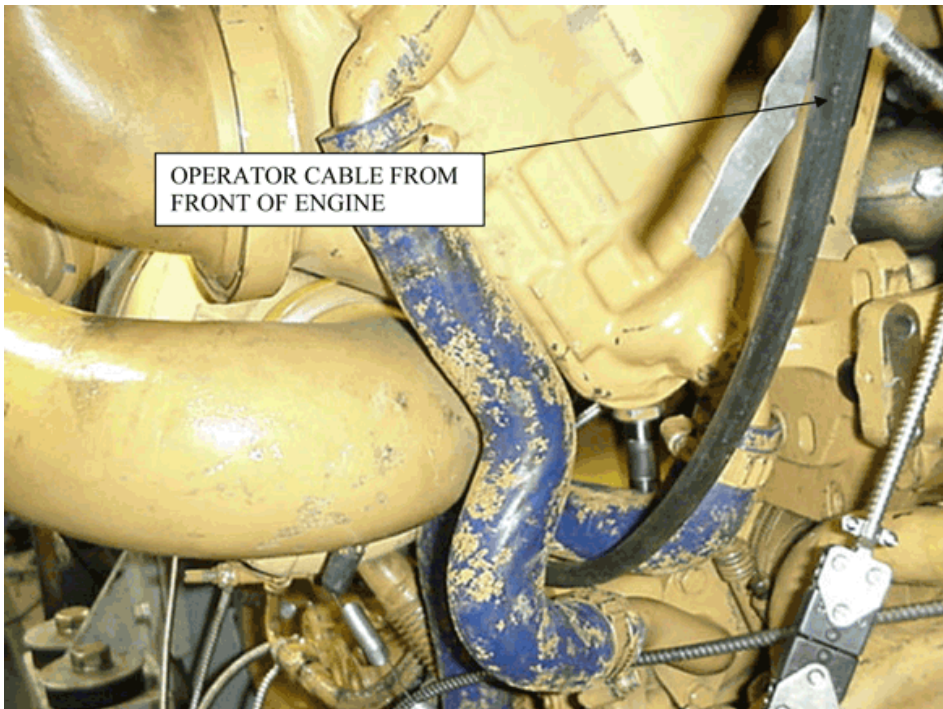
FIG. A5.22 Turbo-Waste-gate Control Cable
