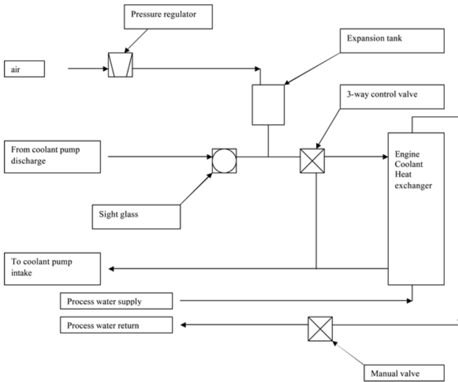
FIG. X1.3 Coolant System (Typical)
