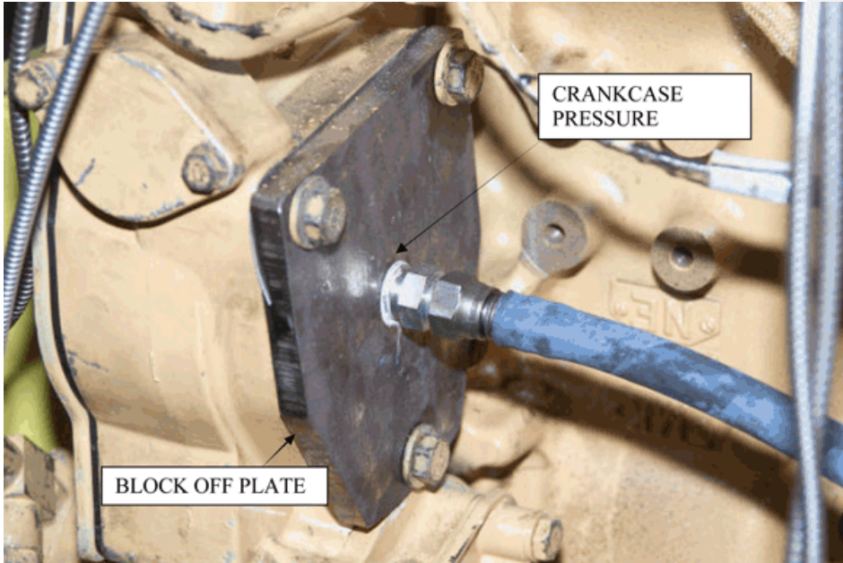
FIG. A5.6 Compressor Block-off Plate and Crankcase Pressure Balance Connection
