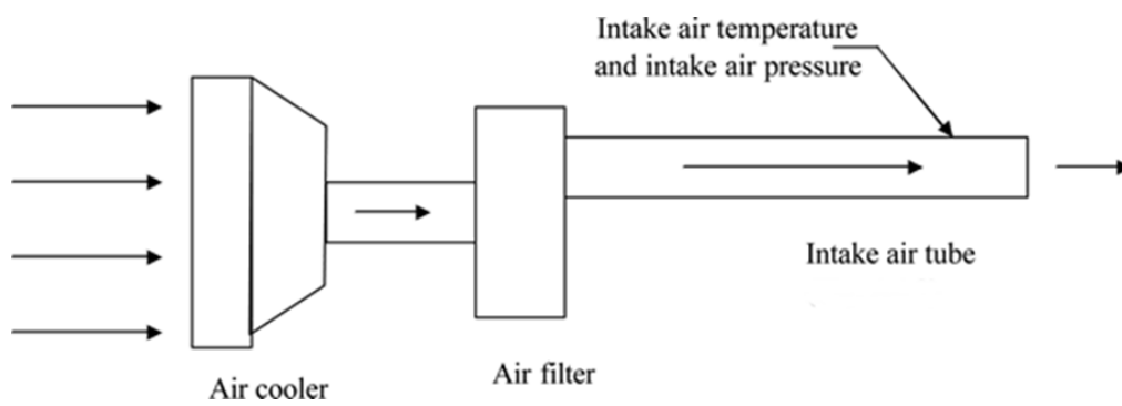
FIG. X1.1 Intake Air System (Typical)
