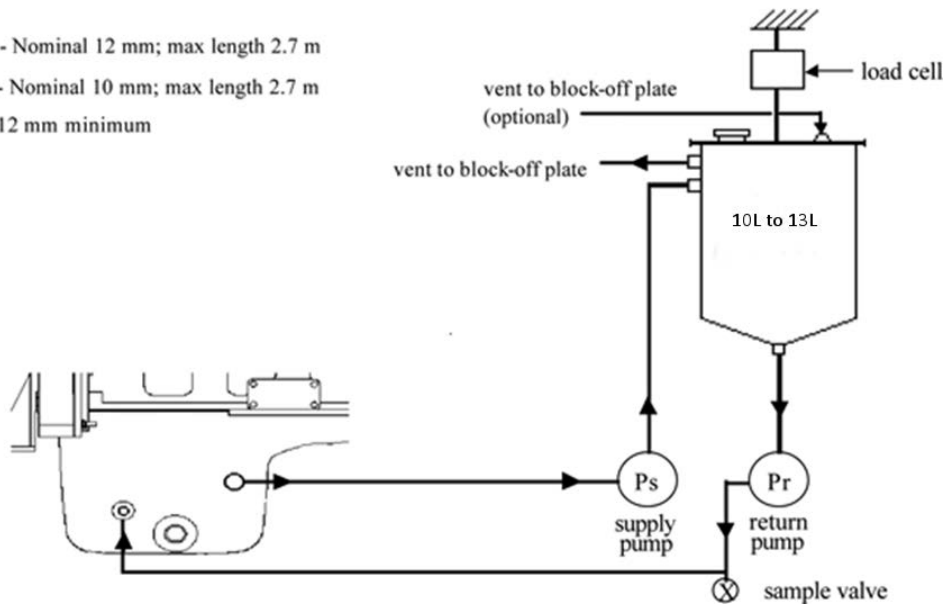
FIG. A6.1 External Oil System
