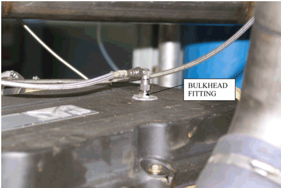
FIG. A5.12 Crankspace-Pressure Connection
