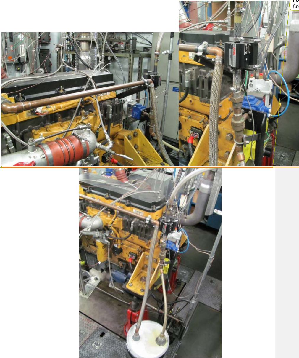
FIG. A5.11 Blowby Flow and Crankcase Pressure Control System
