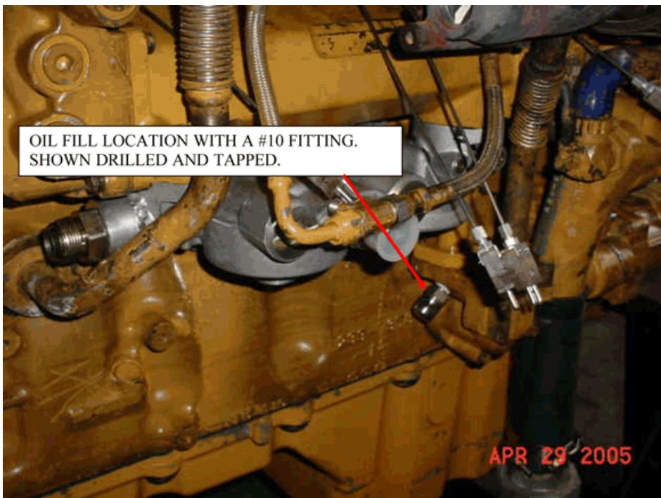
FIG. A5.24 Pressurized Oil-Fill Location
