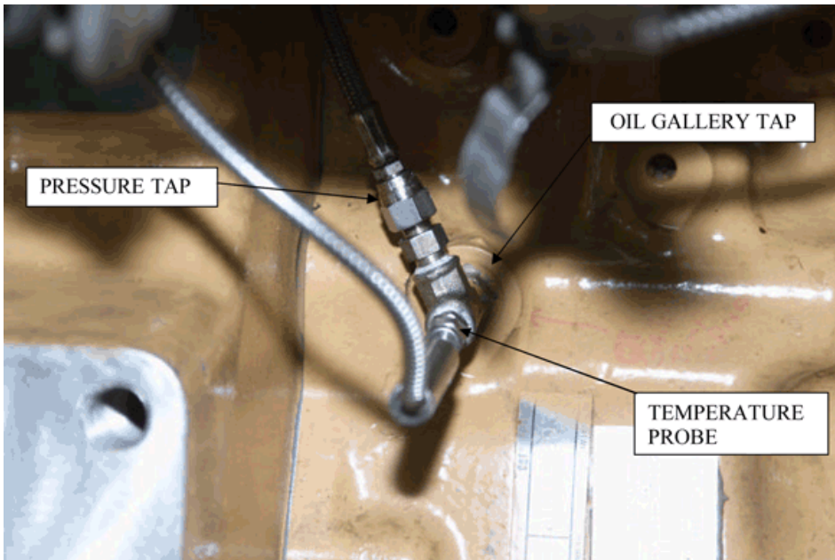
FIG. A5.15 Oil-Gallery Pressure and Temperature Measurement
