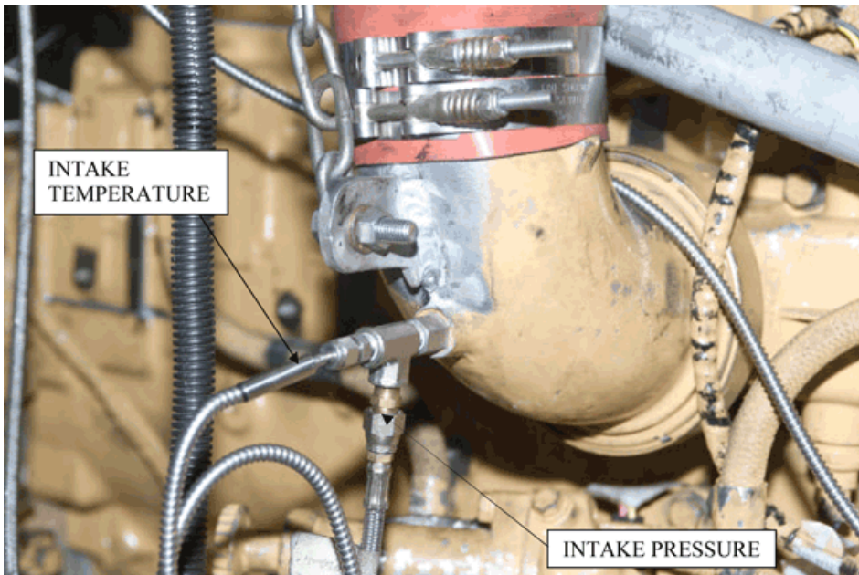
FIG. A5.17 Intake-Manifold Pressure and Temperature Measurement
