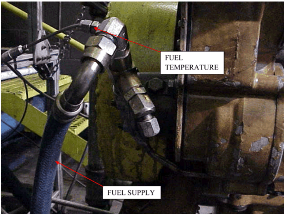
FIG. A5.16 Fuel-to-Engine Temperature Measurement
