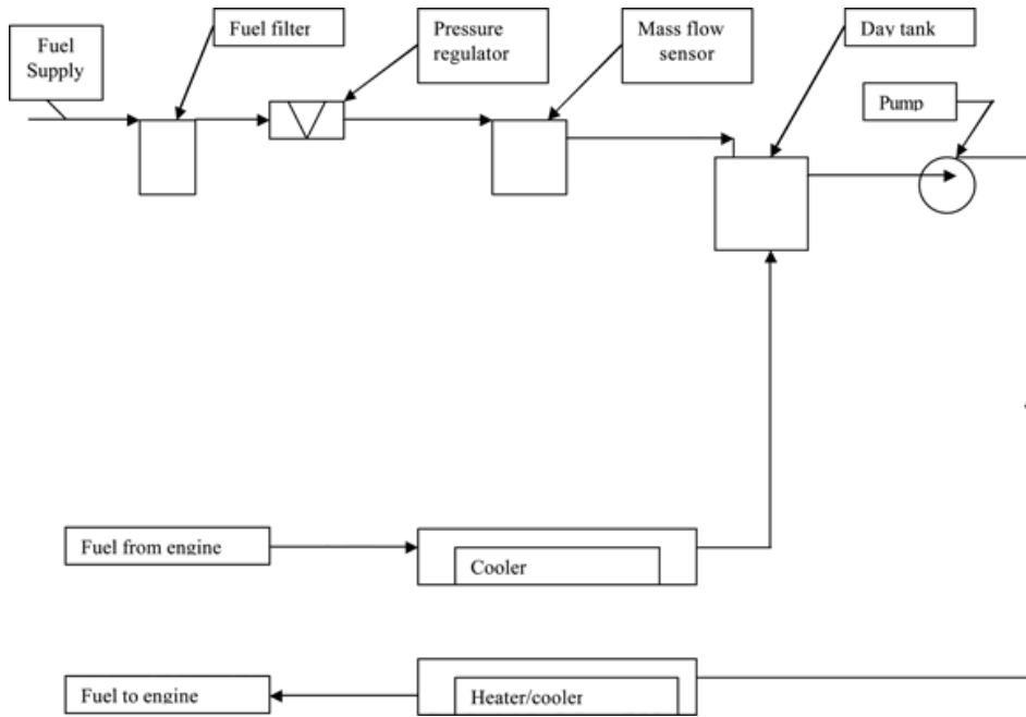
FIG. X1.2 Fuel System (Typical)
