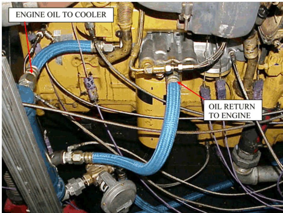
FIG. A4.1 Remote Oil Heat Exchanger
