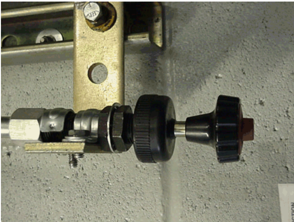
FIG. A5.23 Manual Adjuster for Turbo Waste-gate Control
