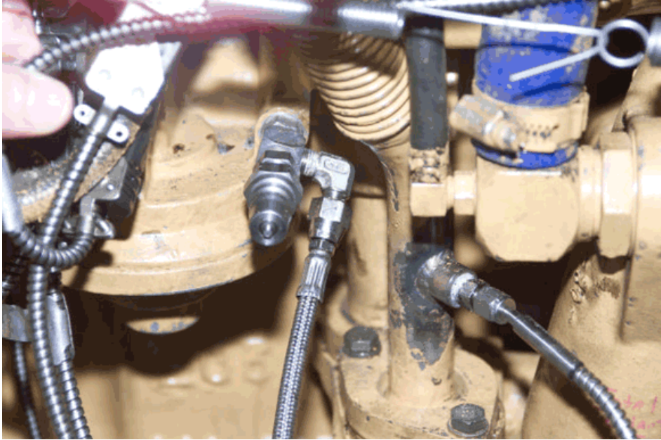
FIG. A5.9 Port for Oil Filter Inlet Pressure
