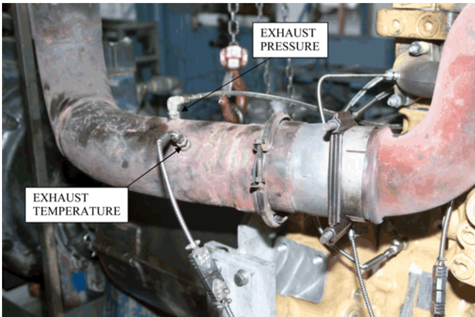
FIG. A5.8 Exhaust Tube
