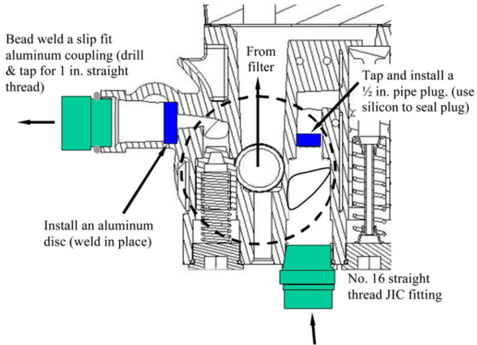
FIG. A4.3 Filter Base Modifications
