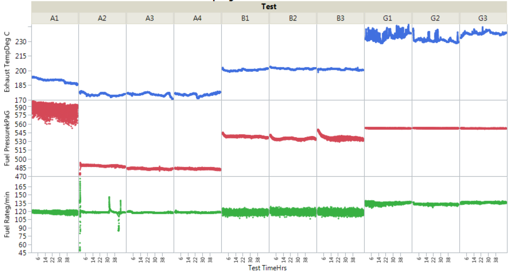
Exhaust TempDeg C & 2 more vs. Test TimeHrs
