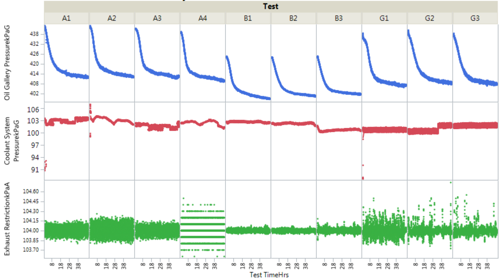
Oil Gallery PressurekPaG & 2 more vs. Test TimeHrs
