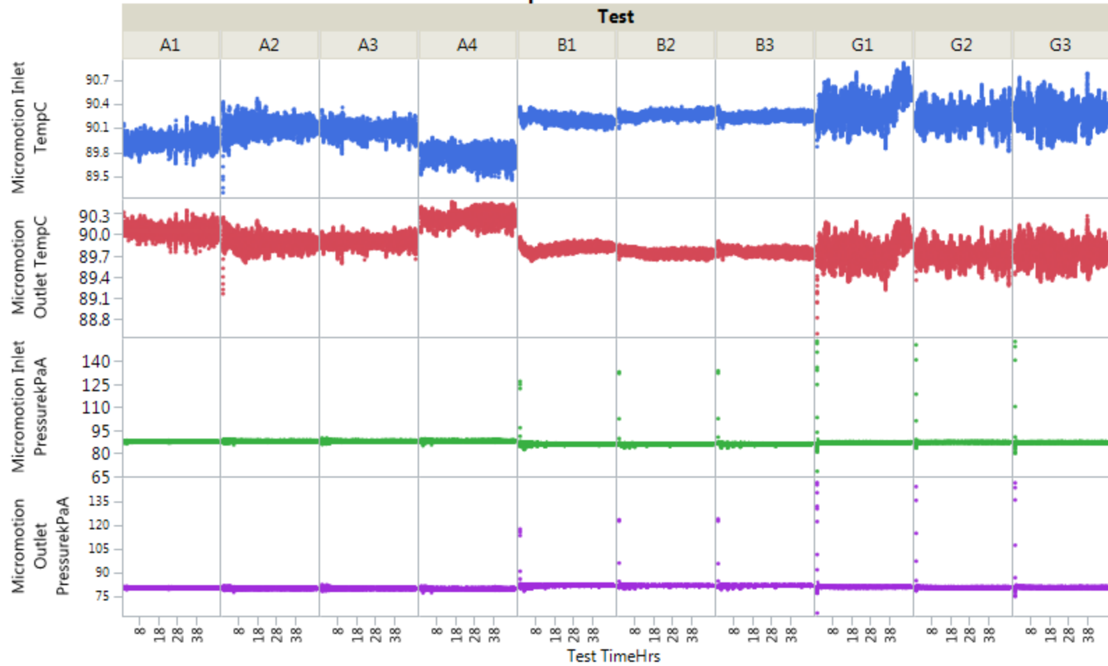
Micromotion Inlet TempC & 3 more vs. Test TimeHrs
