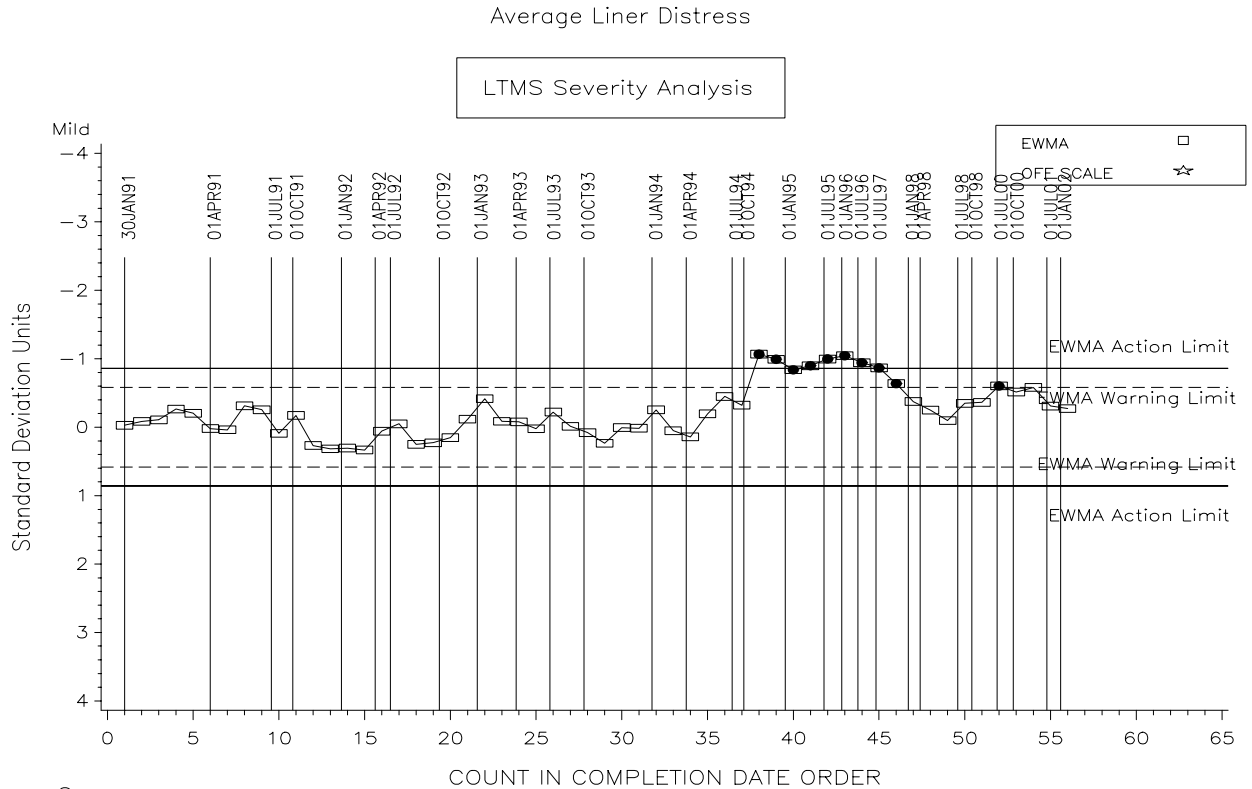
Figure 6 6V92 INDUSTRY OPERATIONALLY VALID DATA
