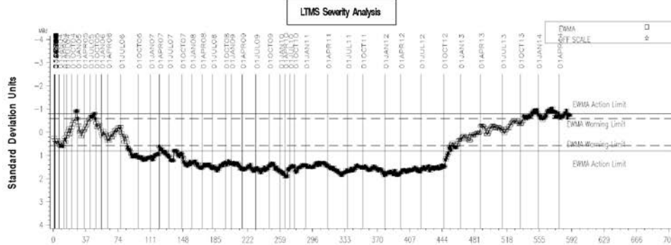
REFERENCE VAMAC G VOLUME CHANGE AVERAGE
